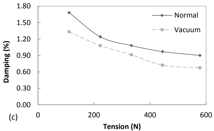
Figure 3.4.4.8 Comparison of damping for 0.3048m carbon fiber cables in air and in vacuum (a)
