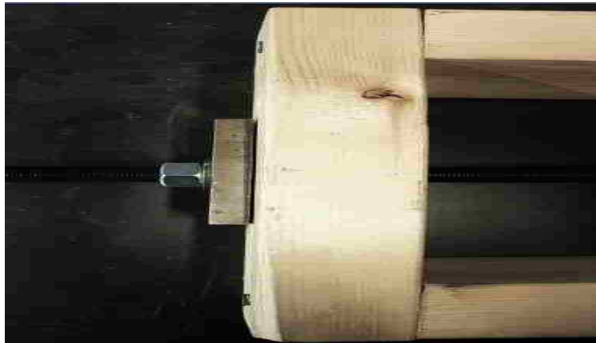
Figure 3.2.2 Tension applying fixture
