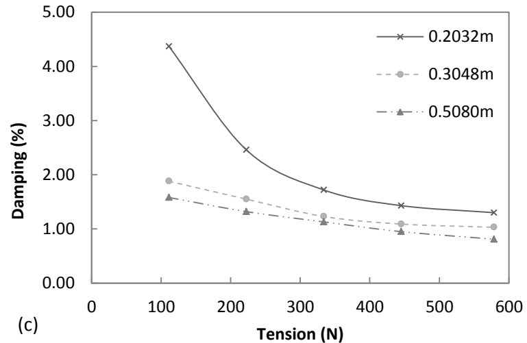
Figure 3.4.1.8 Damping versus tension for cables at a temperature of 4 °C (a) 20.71turns/m (b) 41.42turns/m (c) 62.13turns/m cables
