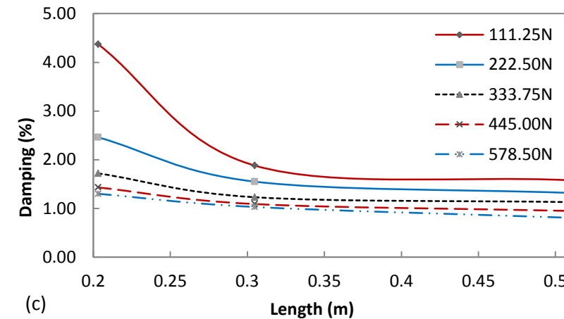
Figure 3.4.2.2 Cable damping versus length for cables at 4°C (a) 20.71turns/m (b) 41.42turns/m (c) 62.13turns/m cables
