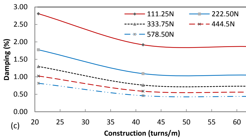
Figure 5.7.2 Cable damping versus cable construction (a) 0.2032m (b) 0.3048m (c) 0.5080m cables
